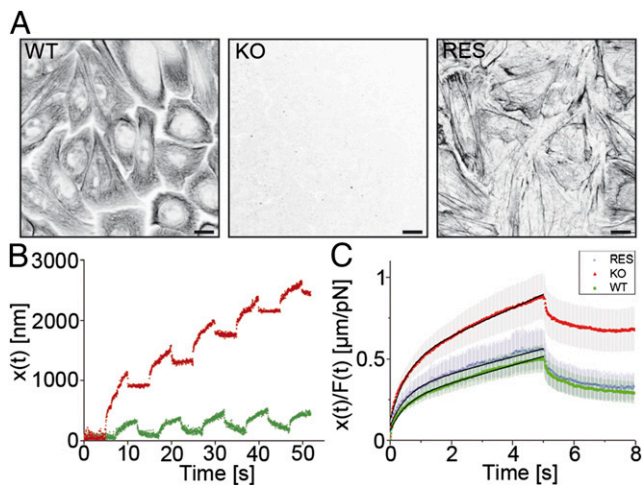
Fig. 5. Keratin network localization and magnetic tweezers analyses. (A) Immunofluorescence micrographs of the keratin network of WT, KO (KtyII -/- ), and K5 rescue (Res) cells. (Scale bars, 10 \mu m.) (B) Example of raw magnetic tweezers data: displacement of the superparamagnetic bead incorporated in the cytoplasm of a WT and a KtyII -/- cell (KO) following the application of 5-s force pulses exerted at 10-s intervals. (C) Average overall rescaled peaks recorded on the three phenotypes as a function of time ( n_{WT} = 40 for 9 cells; n_{KO} = 39 for 10 cells; n_{RES} = 22 for 6 cells). In black, fits of Eq. 3. Error bars are SEM.
